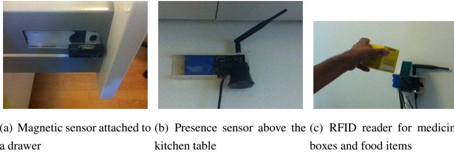
Figure 3.4: Some sensors used in the smart home lab.
