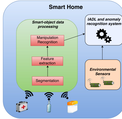
Figure 5.1: General architecture
