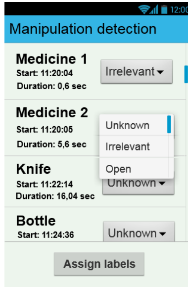
Figure 5.5: Application layout
